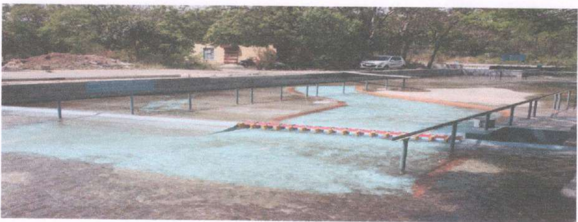
Photo No.4 Jigaon model, CWPRS, Pune
