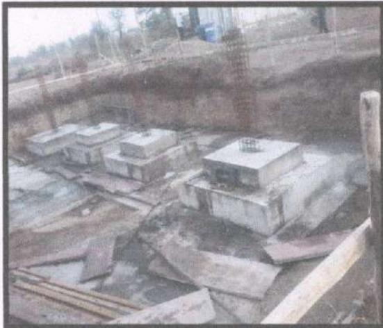
Photo No.1 -Combined footing
