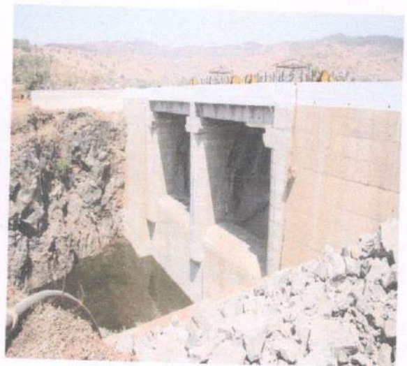
Photo No.6- Ogee spillway
