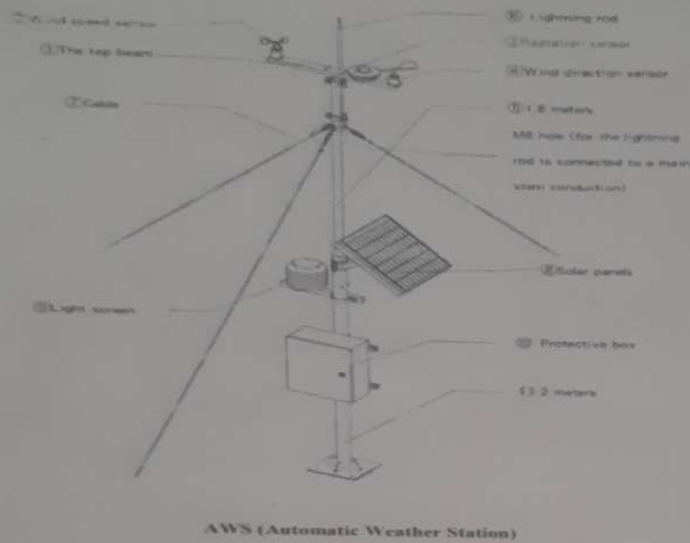
Fig.1: Components of AWS
