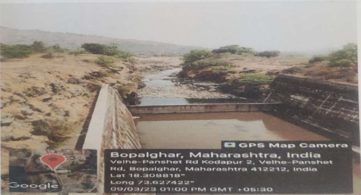
Photo.No.1-Stilling basin & Spillway
