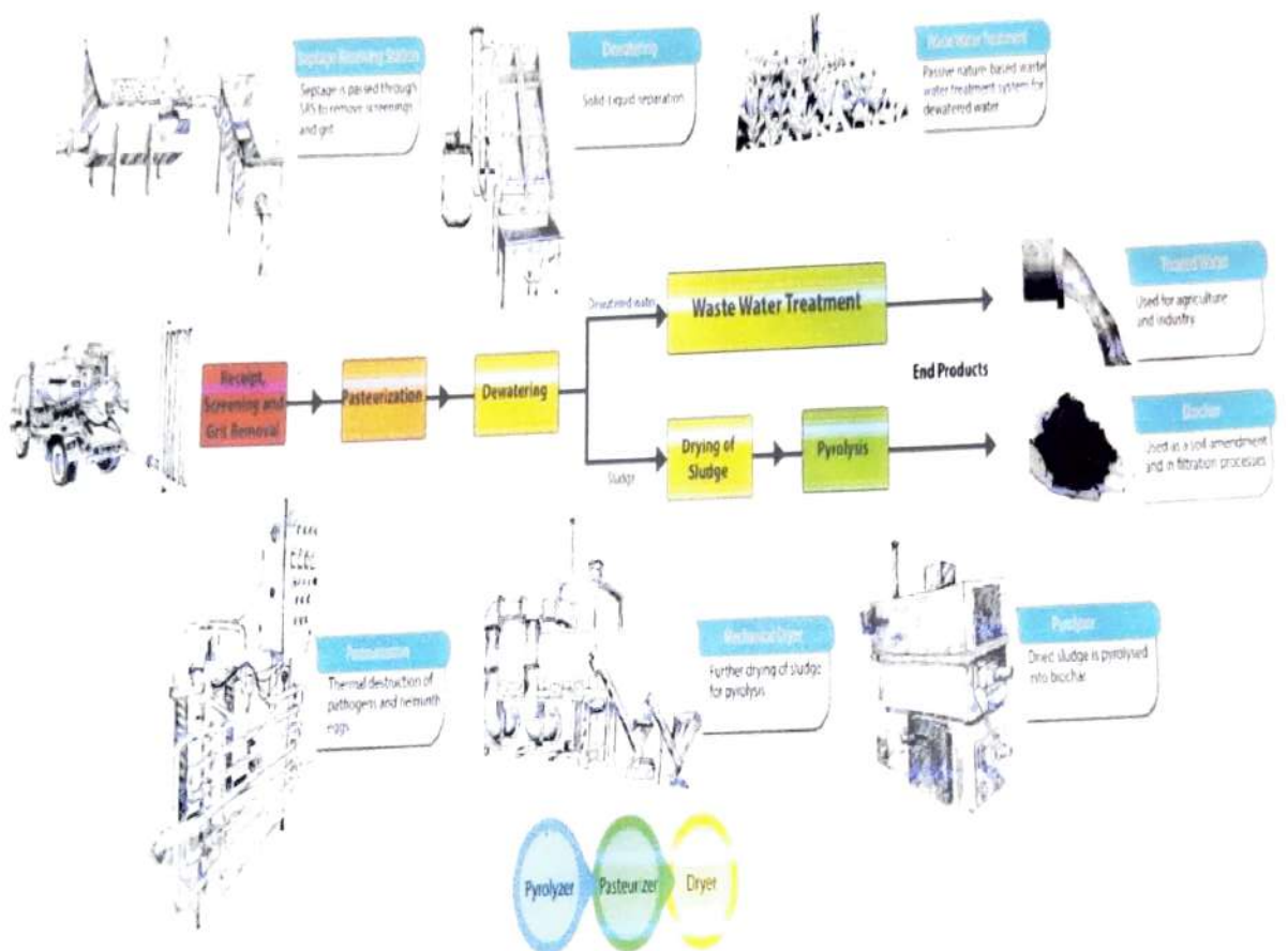
Fig.1 Flow Diagram Of Waste Water Treatment plant
